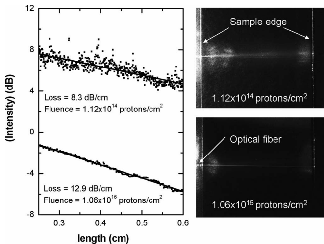
FIG. 3. Loss data measured from the waveguides fabricated with a fluence of 1 \times 10^{14} protons/cm 2 and 1 \times 10^{16} protons/cm 2 . The loss values we obtained ranged from 8.3 to 12.9 dB/cm.
