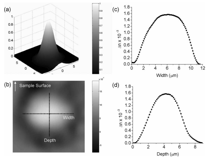
FIG. 2. (a) Near-field mode profile measured from the waveguide fabricated with the highest fluence ( 1 \times 10^{16} protons/cm 2 ). (b) Recovered two-dimensional 2D refractive index profile and line profiles through the center of the mode along the (c) width and (d) depth of the sample.
