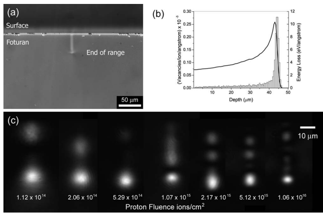
FIG. 1. (a) Optical differential interference contrast image of the Foturan™ sample edge showing a waveguide and the end of range region. (b) SRIM 2003 simulation of 2 MeV protons in Foturan™ (density=2.37 g/cm 3 ) showing the vacancy profile due to nuclear stopping and the ionization profile due to electronic stopping. (c) Optical images of the waveguide mode profiles for seven different proton beam fluences. The laser used for these measurements was a 17 mW, 632.8 nm helium–neon laser.
